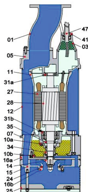
SH22-75kW
