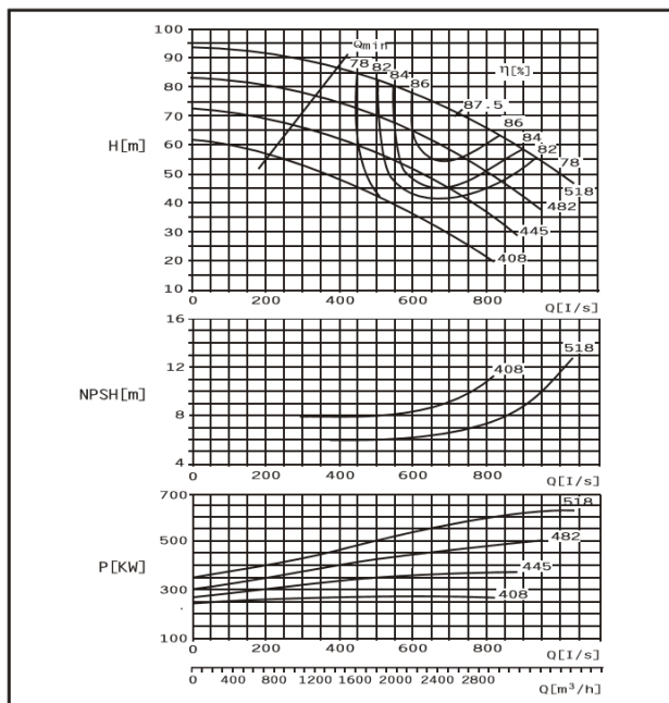
DMC350-510 E
