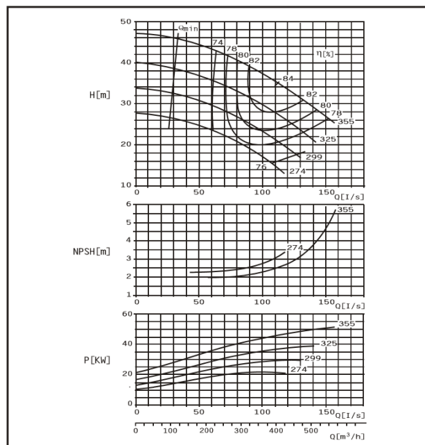
DMC150-360 F
