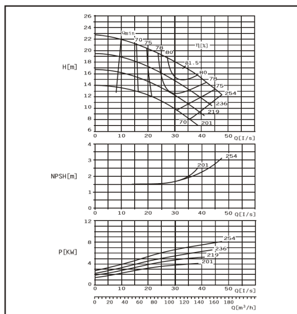
DMC100-250 F
