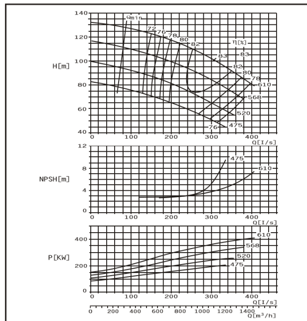
DMC250-600 F
