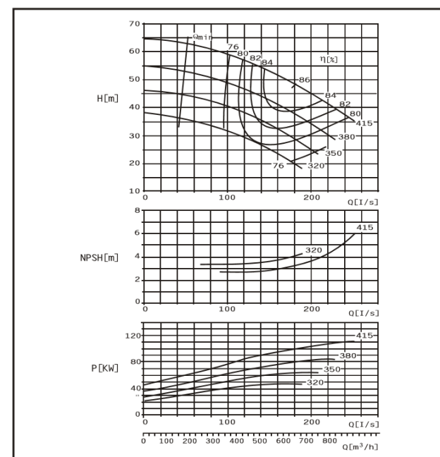
DMC200-420 F
