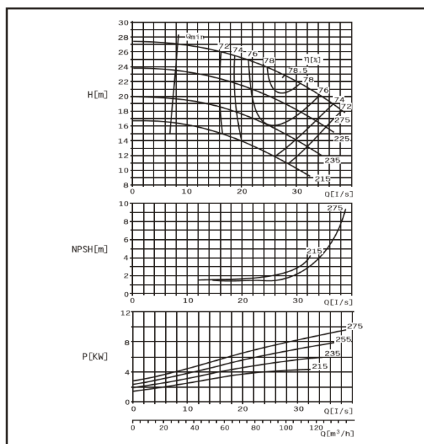
DMC80-270 E
