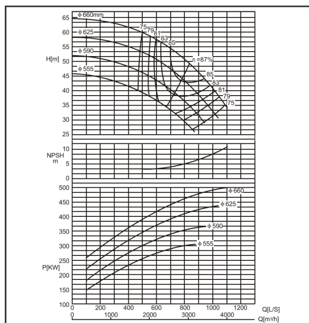
DMC500-700 F
