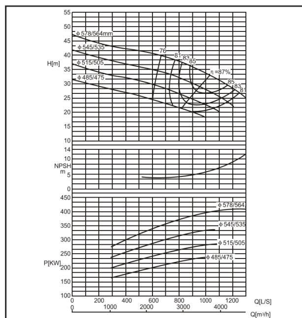
DMC600-620 F
