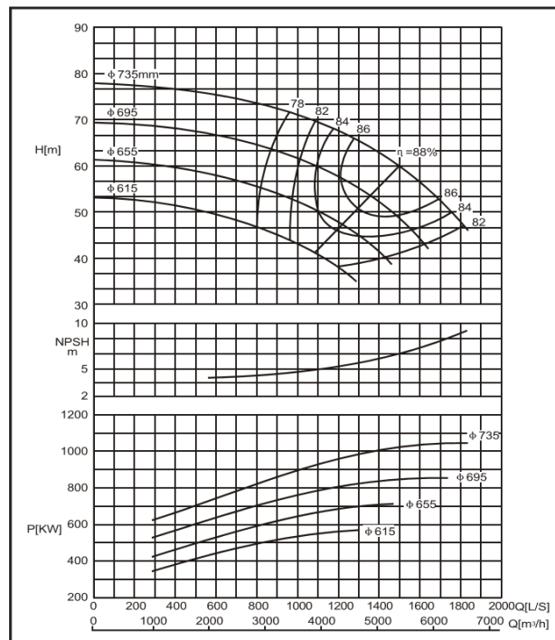
DMC700-820F
