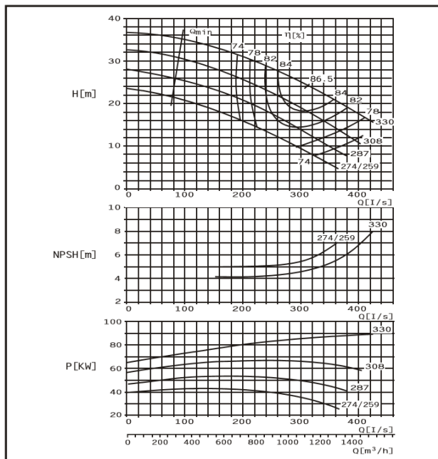
DMC300-300 E
