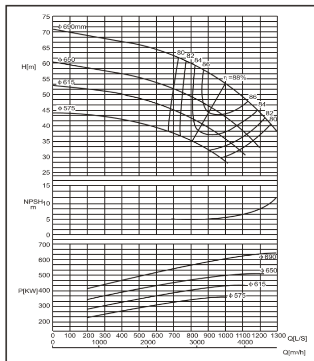
DMC600-710 F
