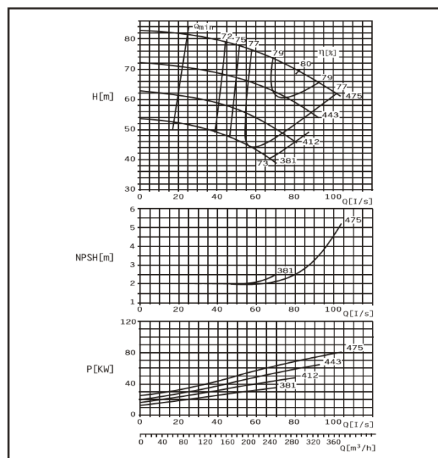
DMC125-500 F
