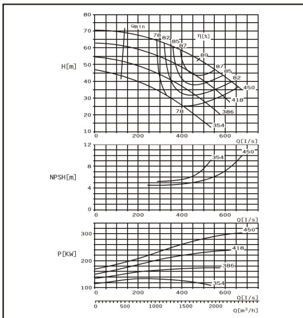
DMC300-435 E
