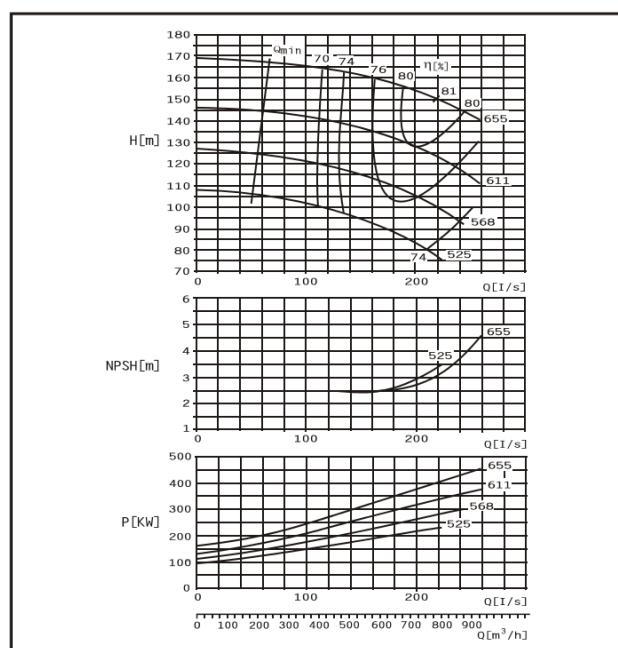
DMC200-670 E
