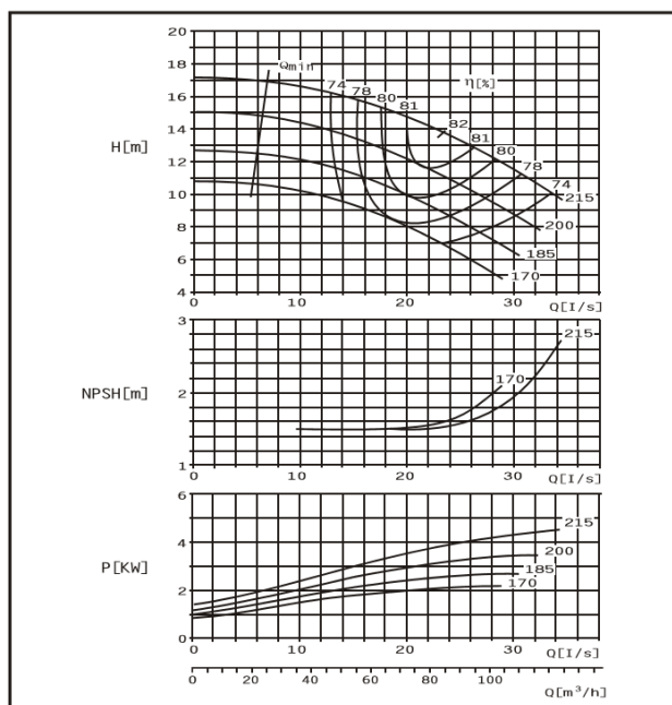
DMC80-210 E
