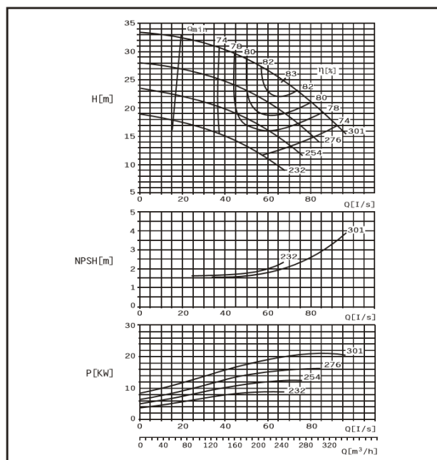
DMC125-290 F
