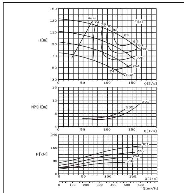
DMC125-290 FG
