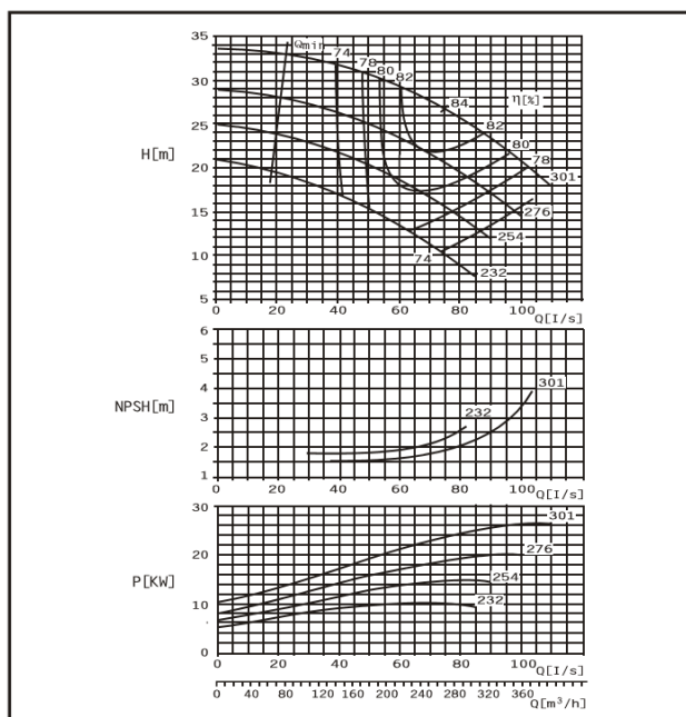
DMC125-290 E
