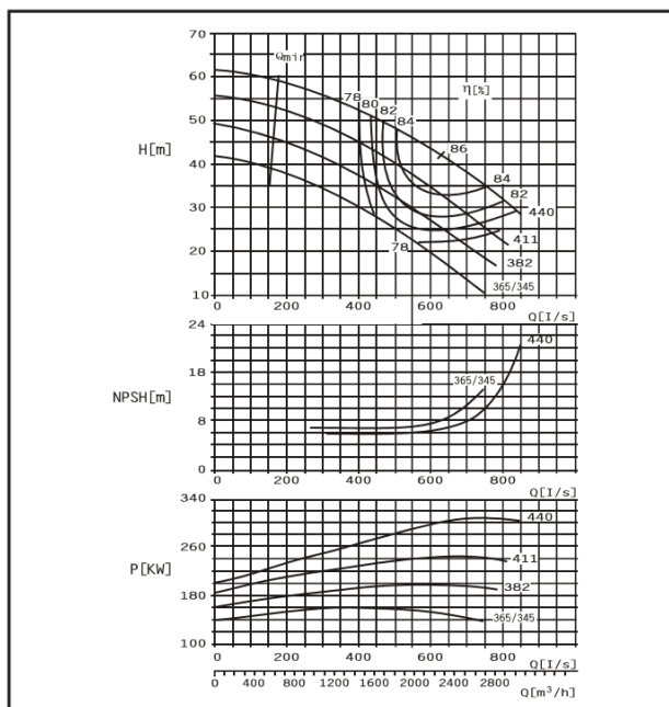
DMC350-430 F
