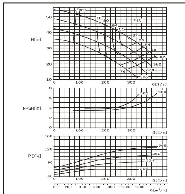
DMC250-370 F
