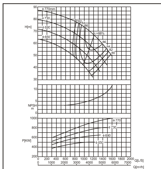
DMC600-830 F
