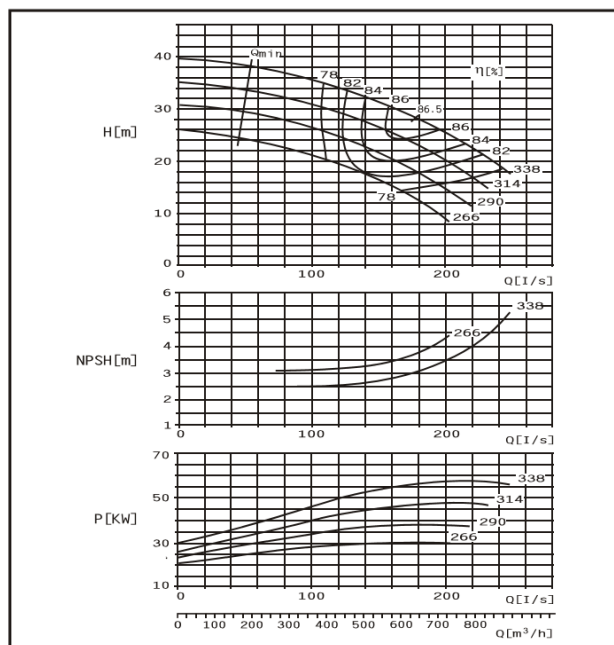
DMC200-320 F
