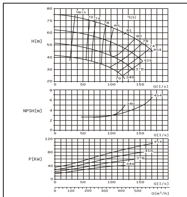
DMC150-460 F
