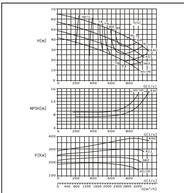
DMC350-430 E
