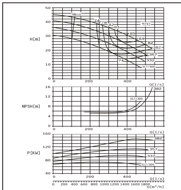
DMC350-360 F
