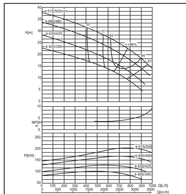
DMC500-510 F
