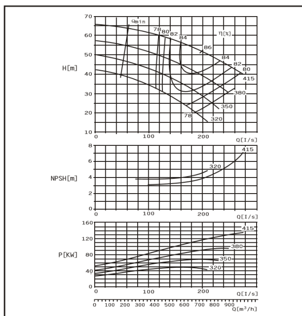
DMC200-420 E
