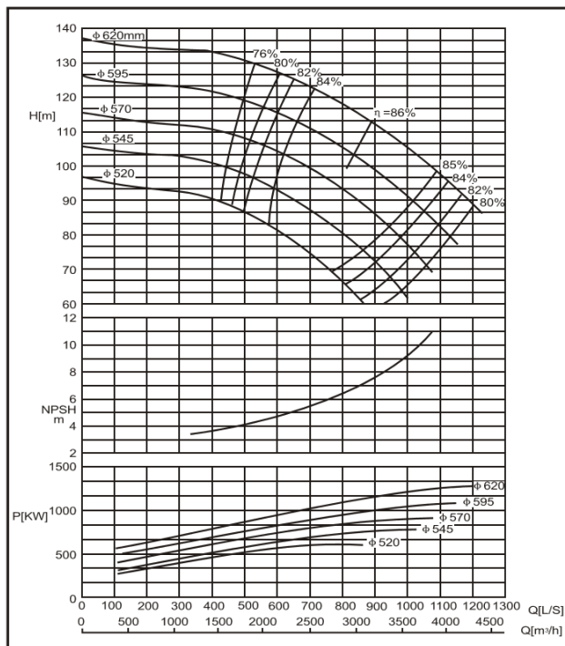
DMC400-620 E
