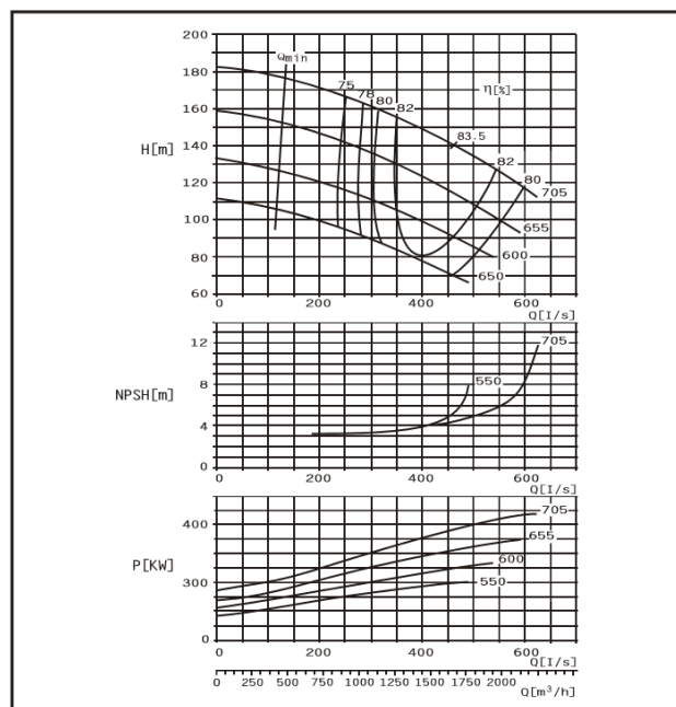
DMC300-700 F
