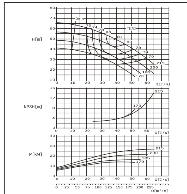
DMC80-210 FG
