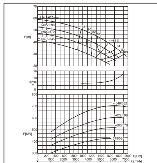
DMC700-710 F
