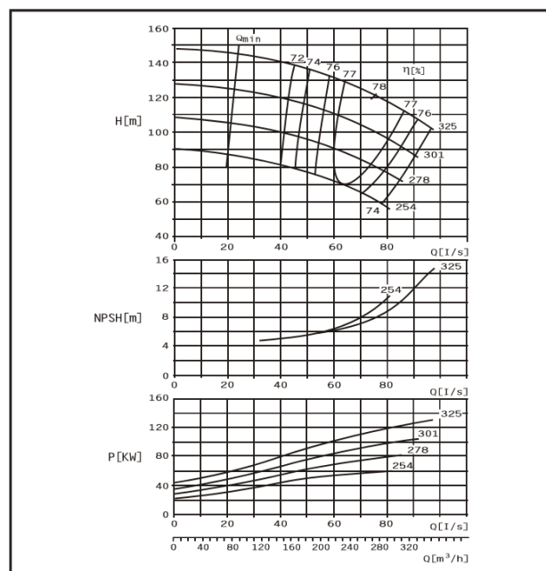
DMC100-310 FG
