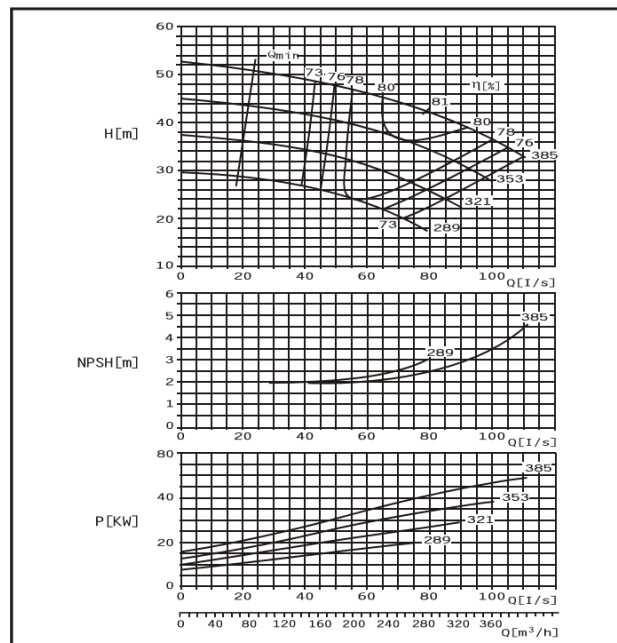
DMC125-365 F
