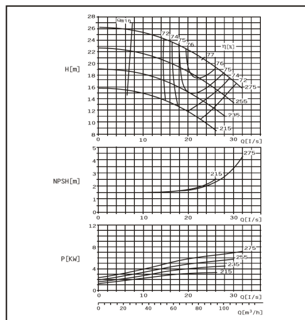
DMC80-270 F
