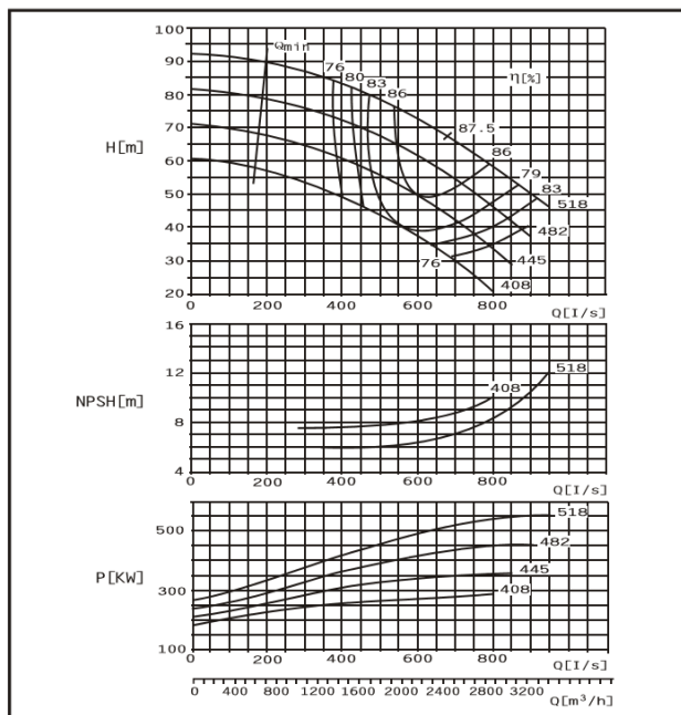
DMC350-510 F
