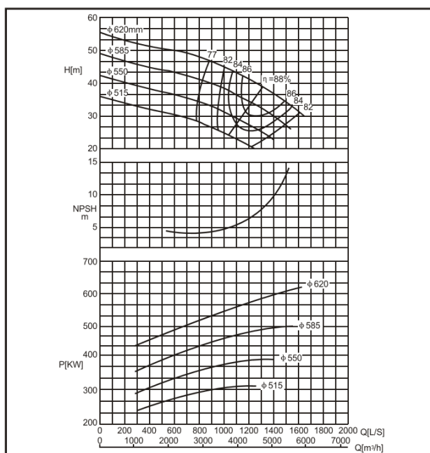
DMC600-620 E
