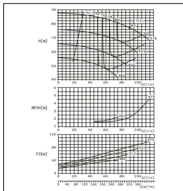
DMC125-500 E
