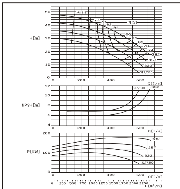
DMC350-360 E
