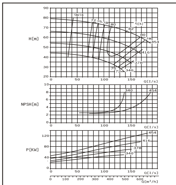
DMC150-460 E
