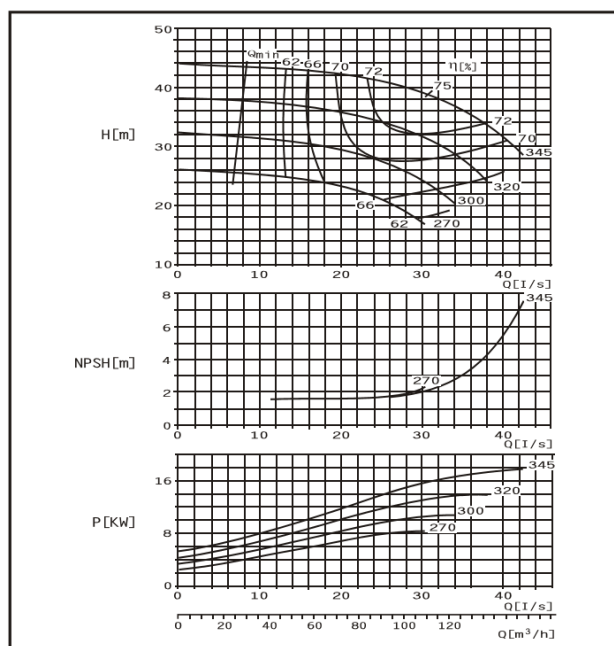
DMC80-370 E
