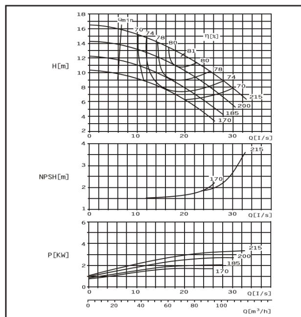
DMC80-210 F
