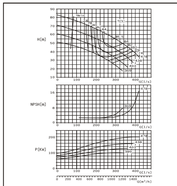
DMC250-480 F
