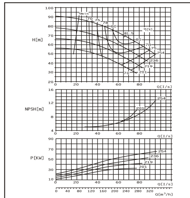
DMC100-250 FG
