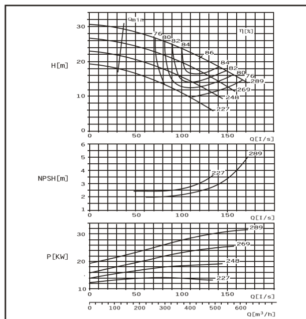
DMC150-290 E
