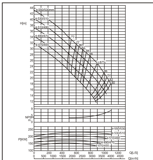
DMC500-510 E
