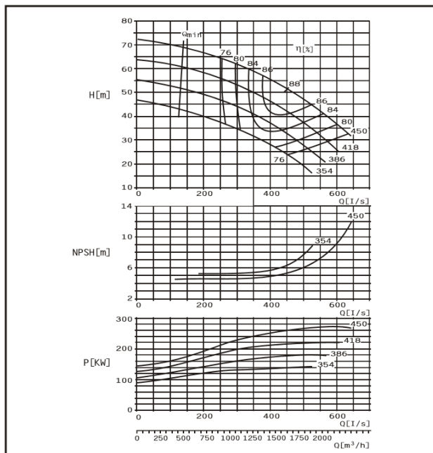
DMC300-435 F
