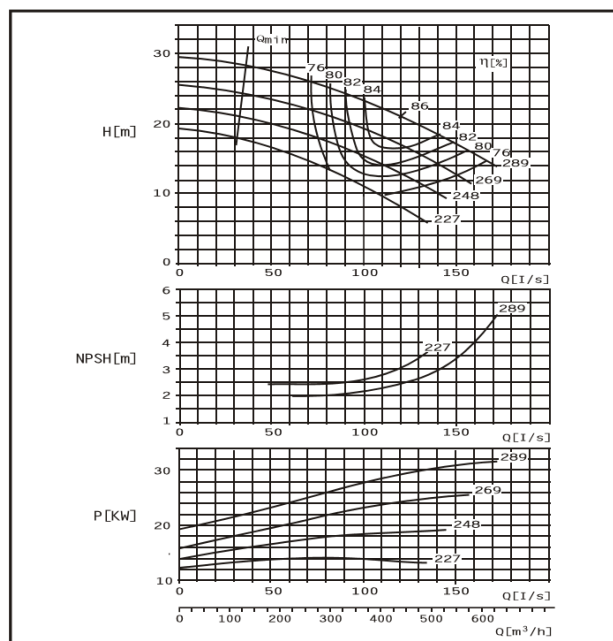
DMC150-290 F
