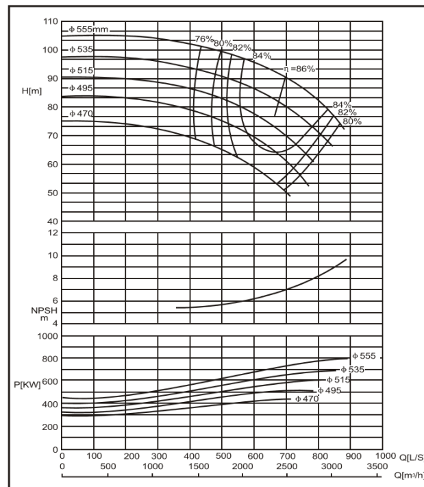
DMC400-620 F
