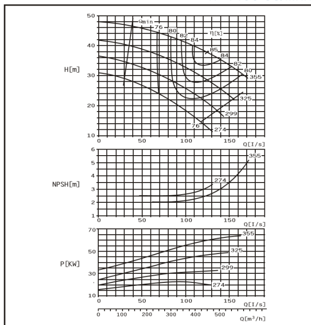
DMC150-360 E
