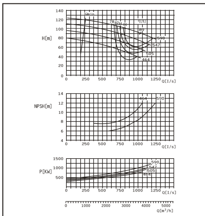
DMC350-590 E
