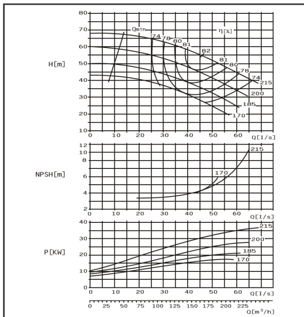
DMC80-210 EG
