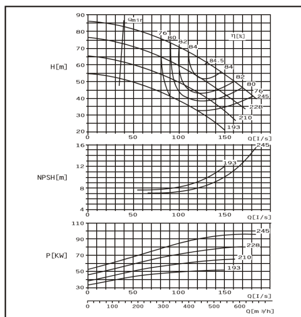
DMC125-230 FG
