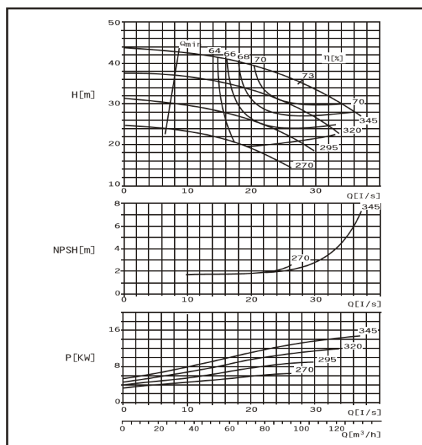
DMC80-370 F
