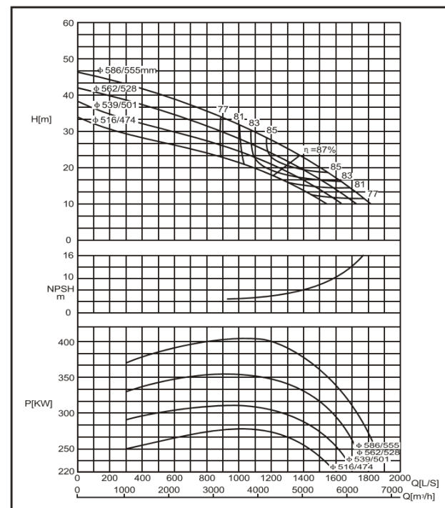
DMC700-590 F
