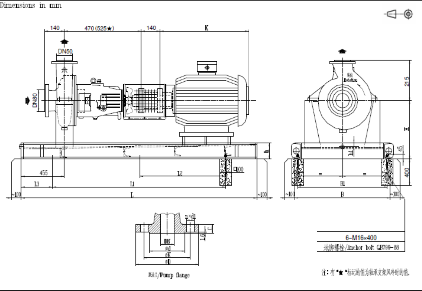
尺寸/DIMENSIONS
