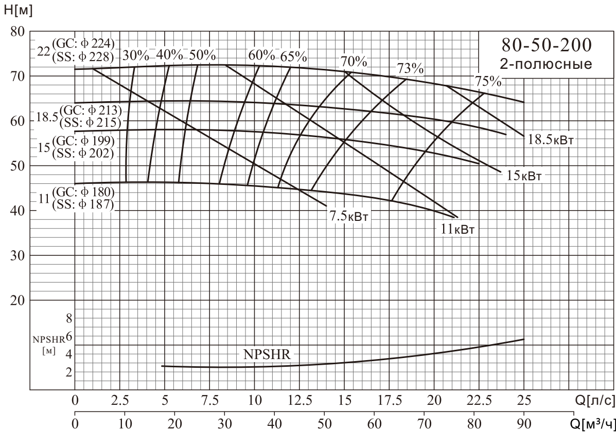
NISO,NIS,NISF 80-50-200/80-50-250
