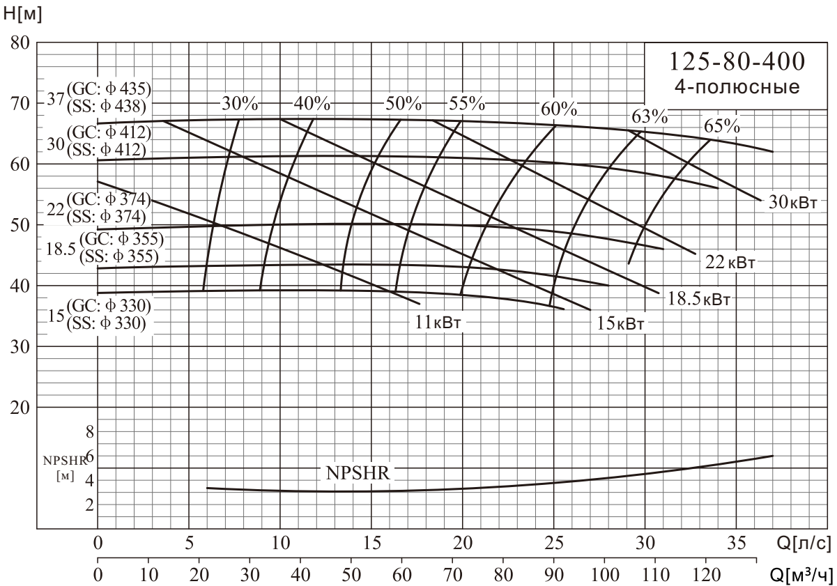
NISO,NIS,NISF 125-80-400/125-100-400
