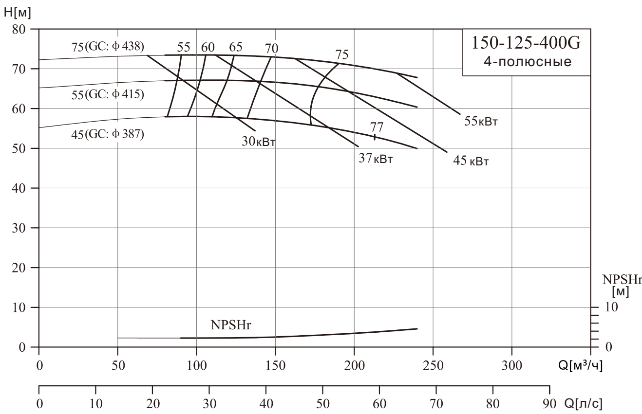
NIS150-125-400G/200-150-250(Q)
