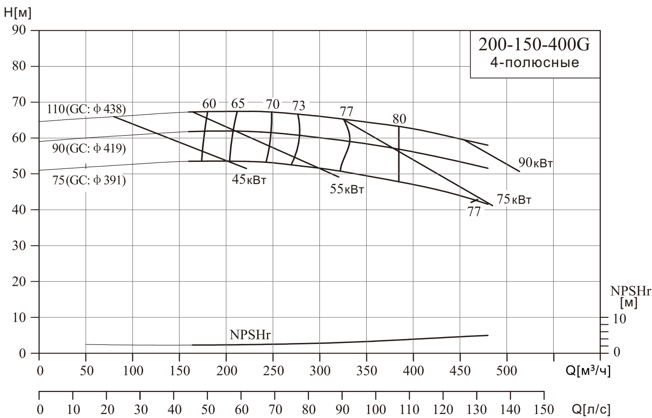
NIS200-150-400G
